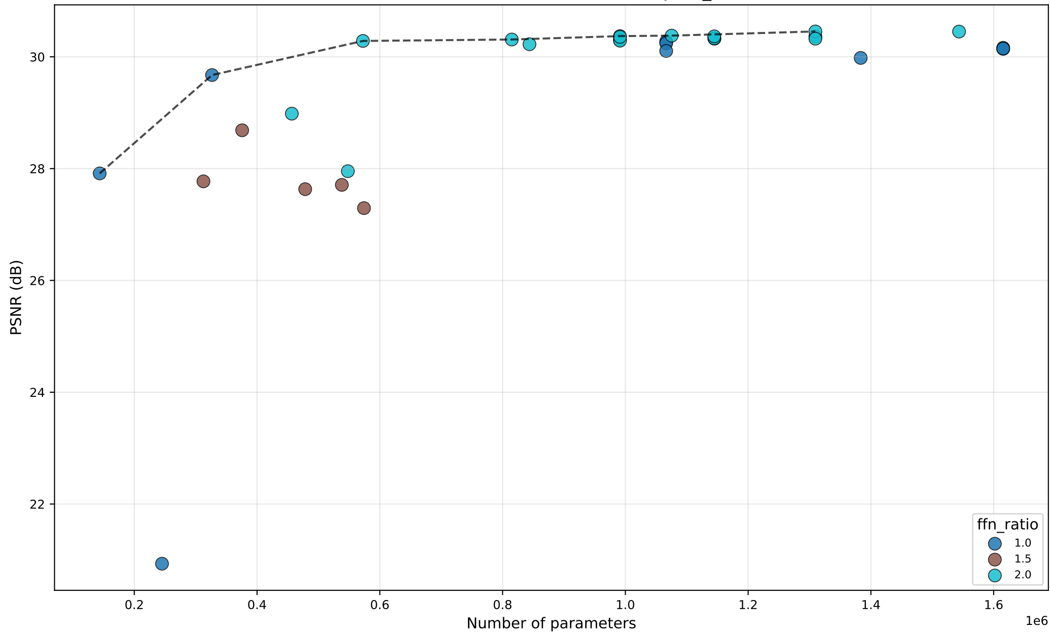
PSNR vs #Params — SRFormer — by ffn_ratio
